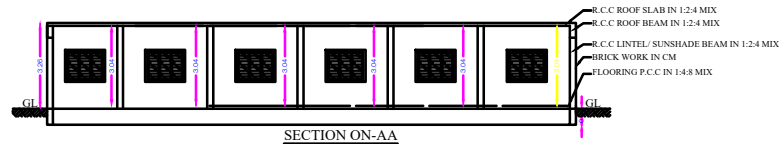
SECTION ON-AA
