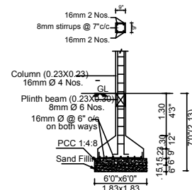
FOUNDATION DETAIL
