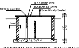
SECTION OF SEPTIC TANK "X Y"
