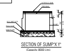
SECTION OF SUMP "X Y"
