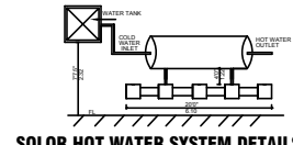
SOLAR HOT WATER SYSTEM DETAILS
