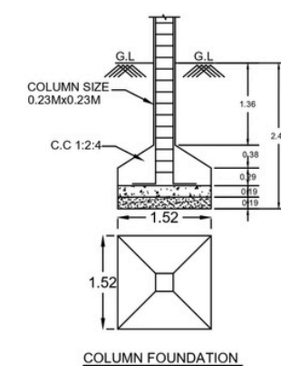
COLUMN FOUNDATION
