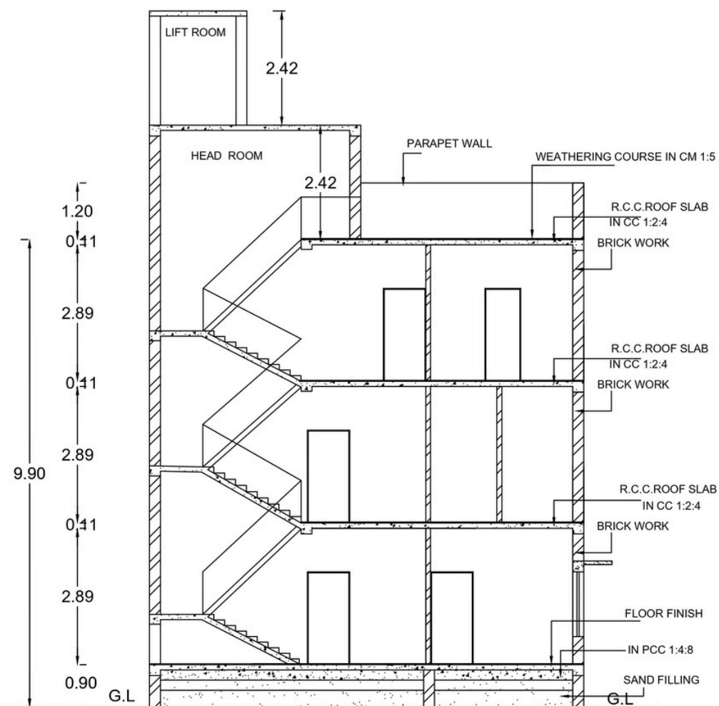
SECTION "AA"
