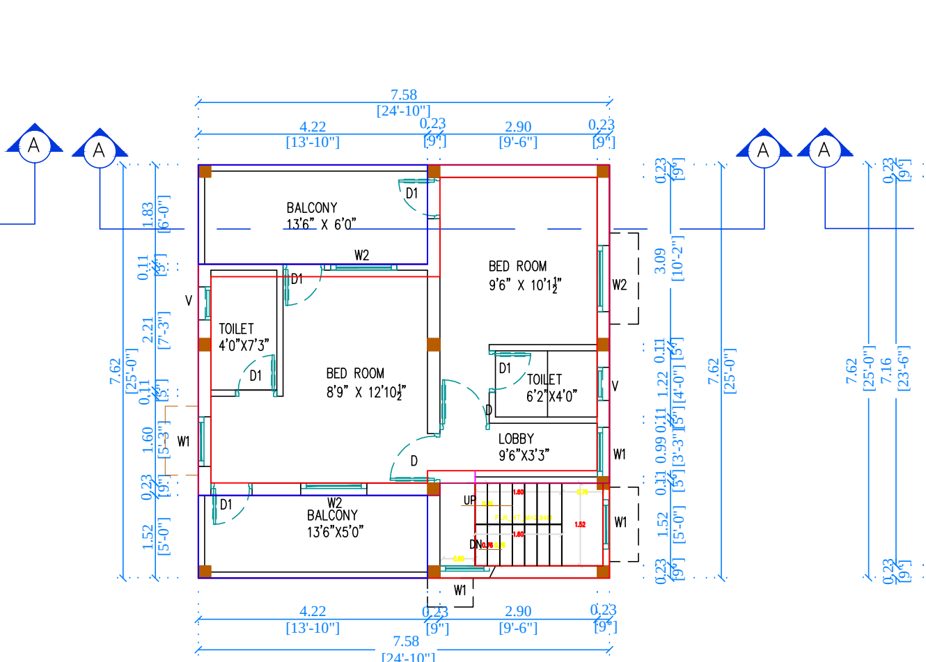
FIRST FLOOR PLAN (PROPOSED)
