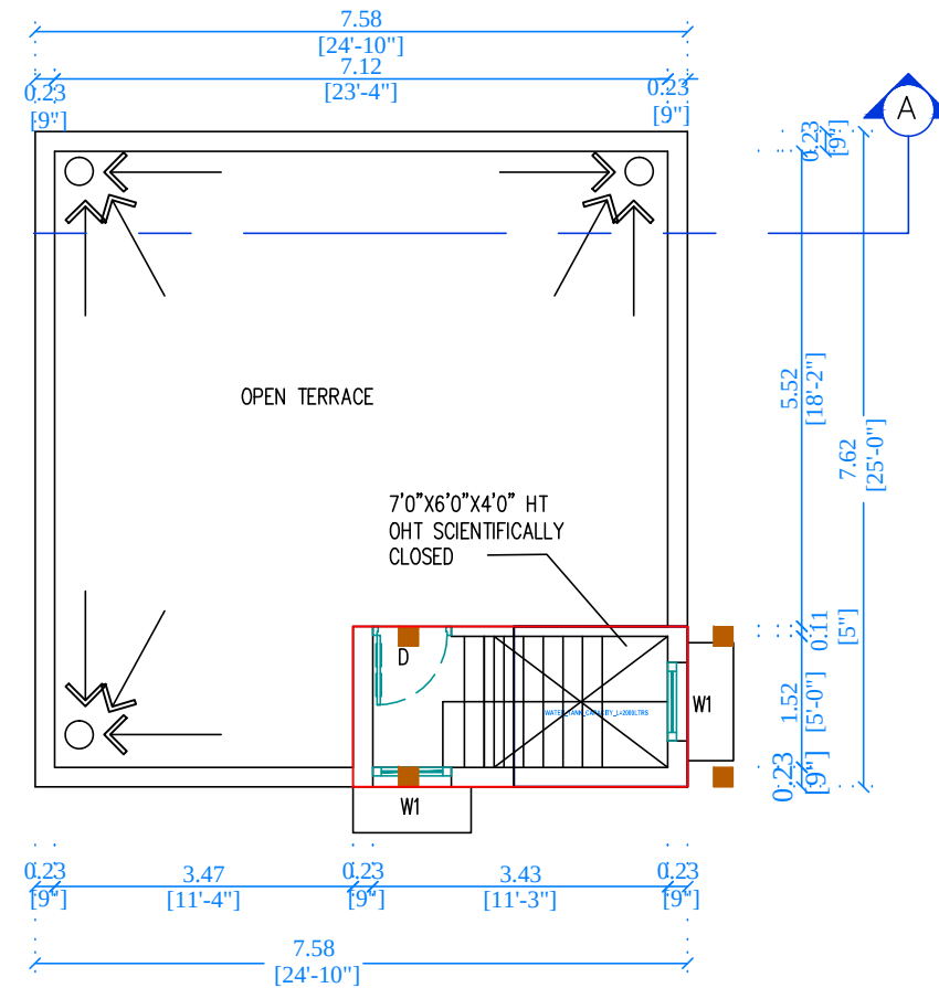
TERRACE FLOOR PLAN (PROPOSED)
