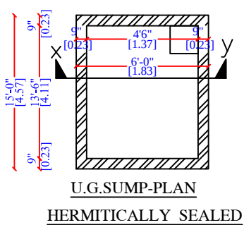
HERMITICALLY SEALED
