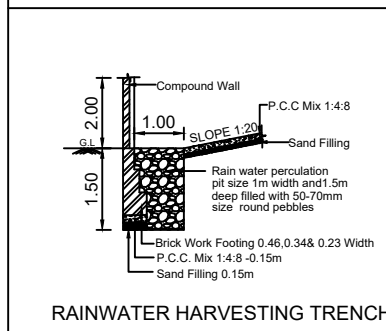
RAINWATER HARVESTING TRENCH
