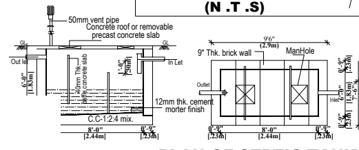
SECTION PLAN OF SEPTIC TANK
