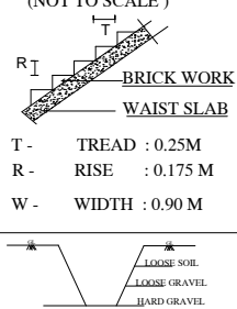
STAIRCASE DETAILS
