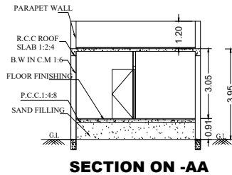
SECTION ON-AA
