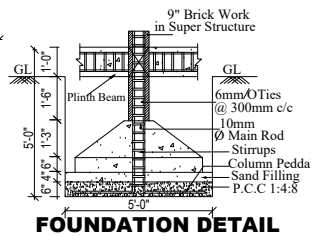
FOUNDATION DETAIL
