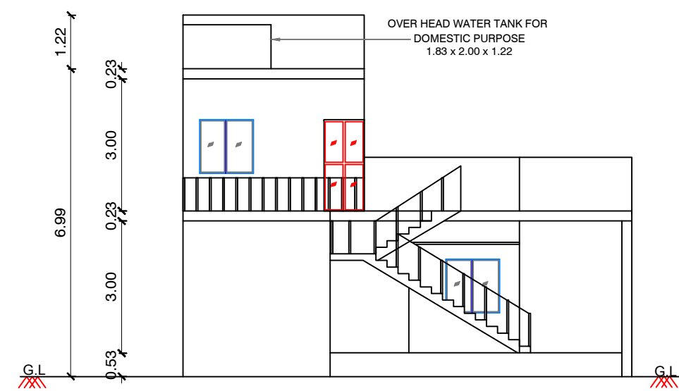
FRONT ELEVATION (PROPOSED)
