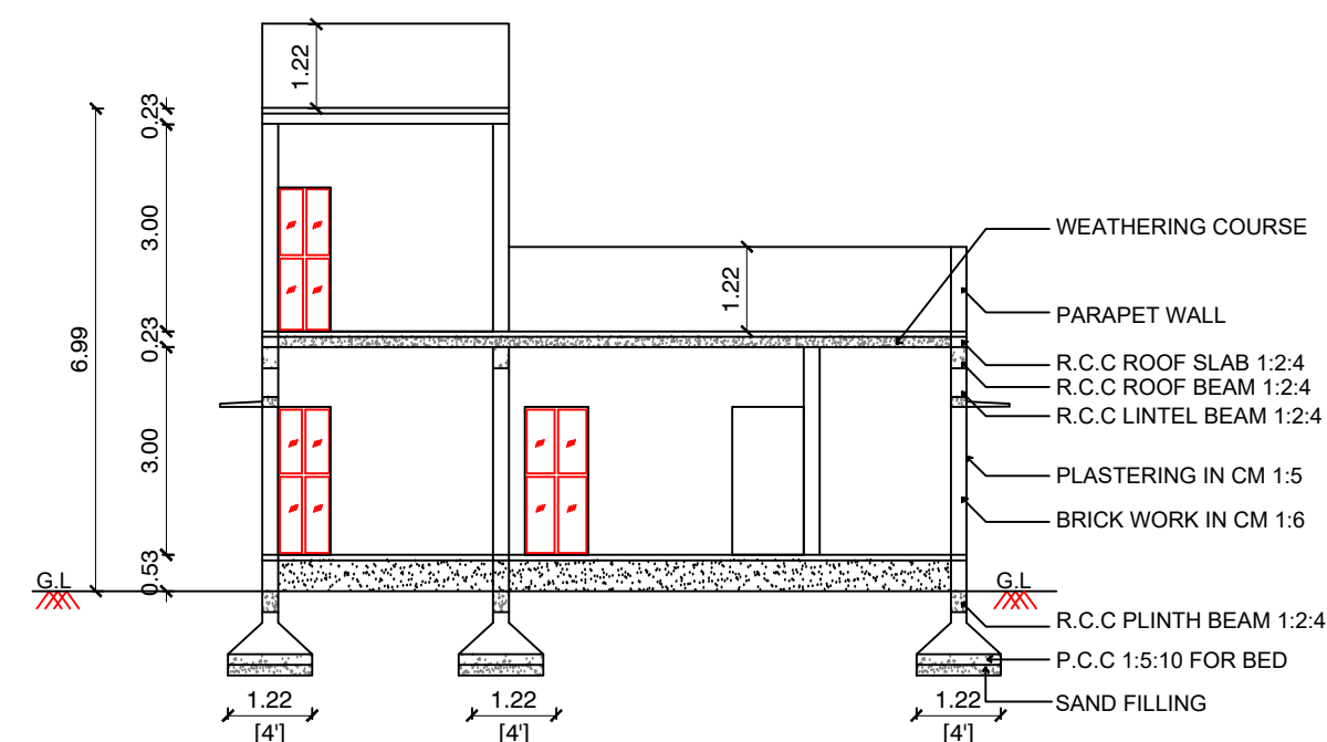
SECTION ON 'AA' (PROPOSED)
