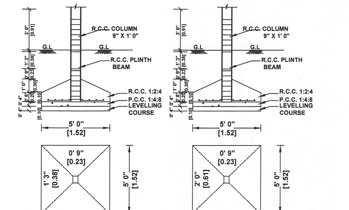
FOUNDATION DETAILS
