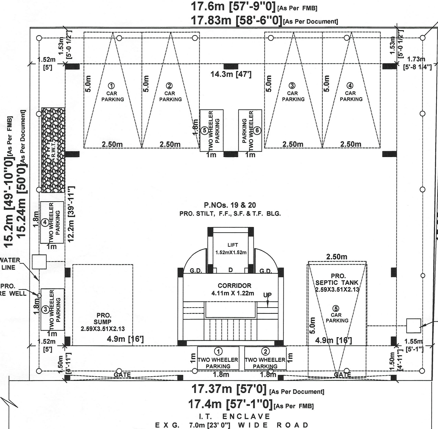
SITE PLAN
