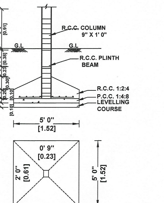
FOUNDATION DETAILS
