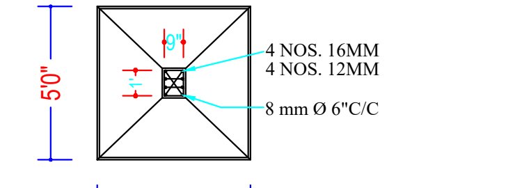
PLAN DETAIL OF COLUMN C1,C2
