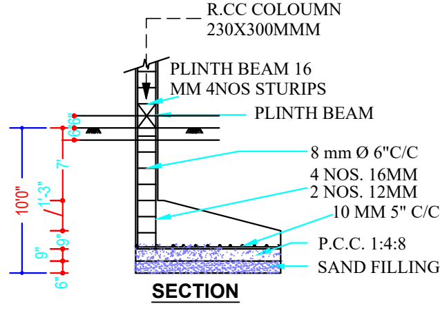
SECTION END WALL FOUNDATION
