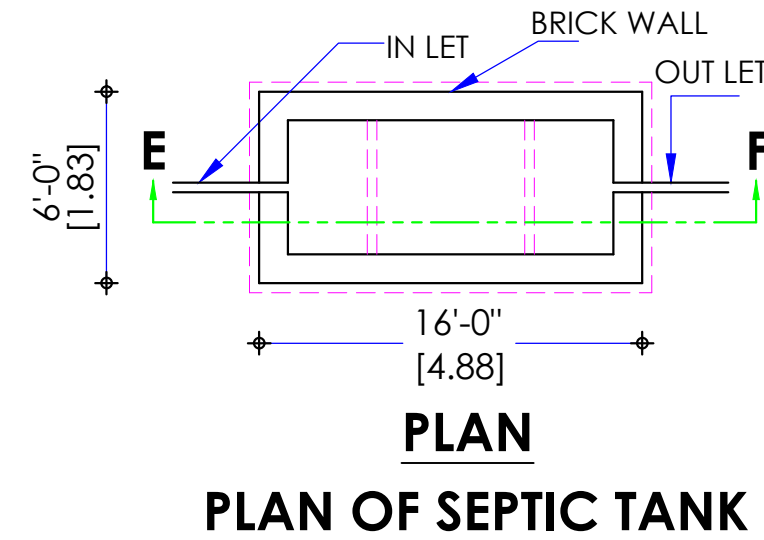
PLAN OF SEPTIC TANK
