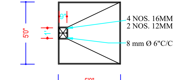
PLAN END WALL FOUNDATION
