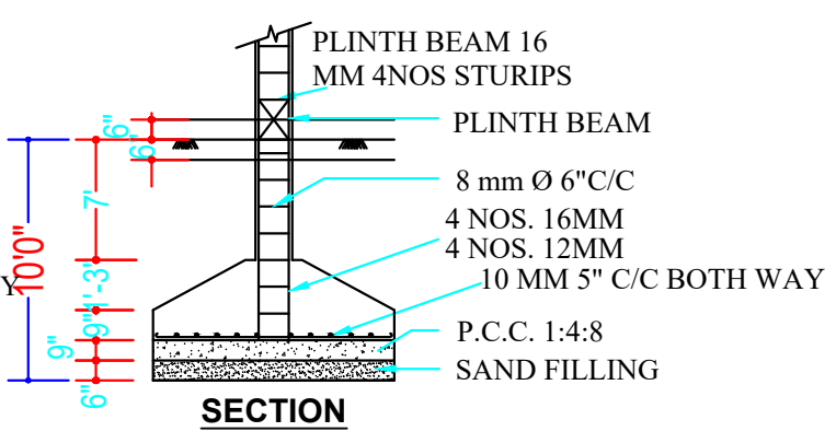
SECTION DETAIL OF COLUMN C1,C2
