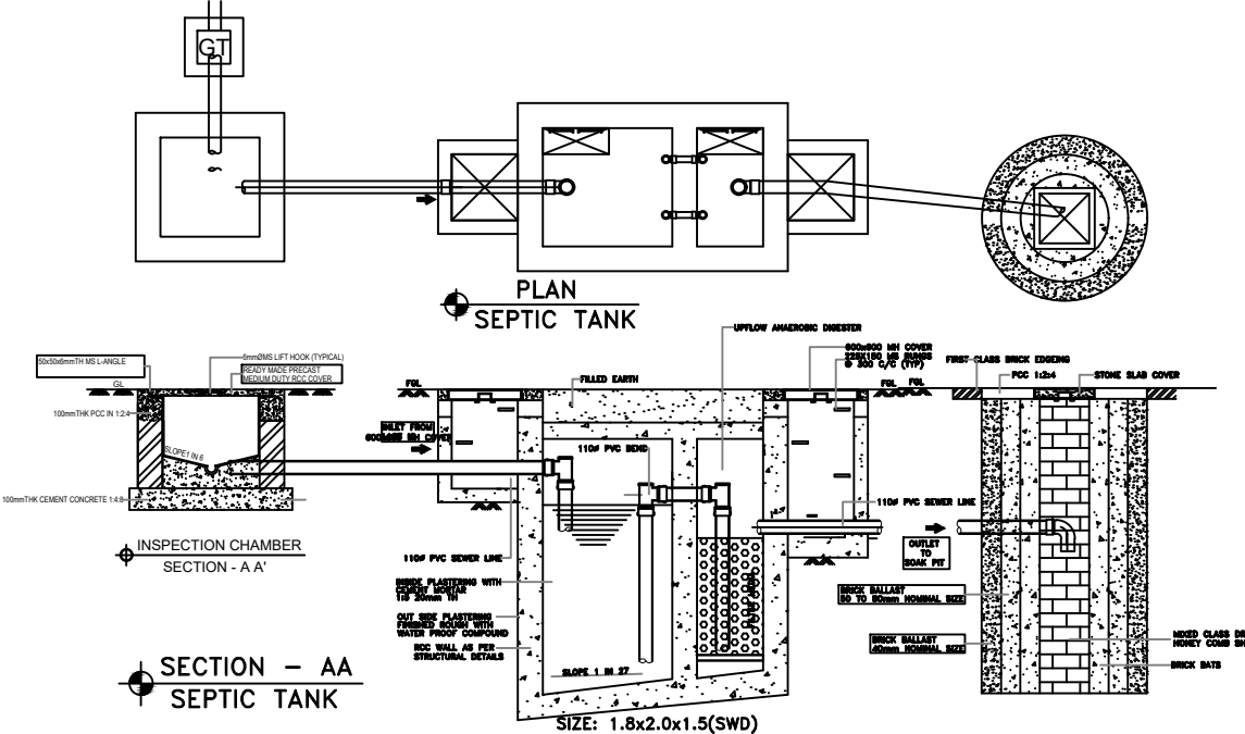
SECTION - AA SEPTIC TANK
