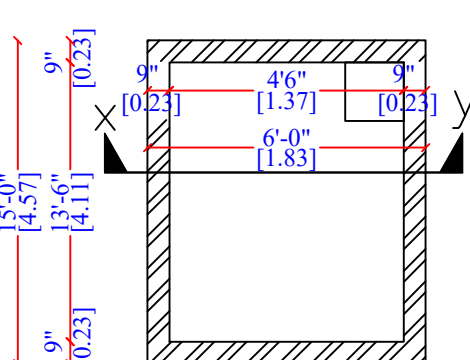
U.G.SUMP-PLAN HERMITICALLY SEALED
