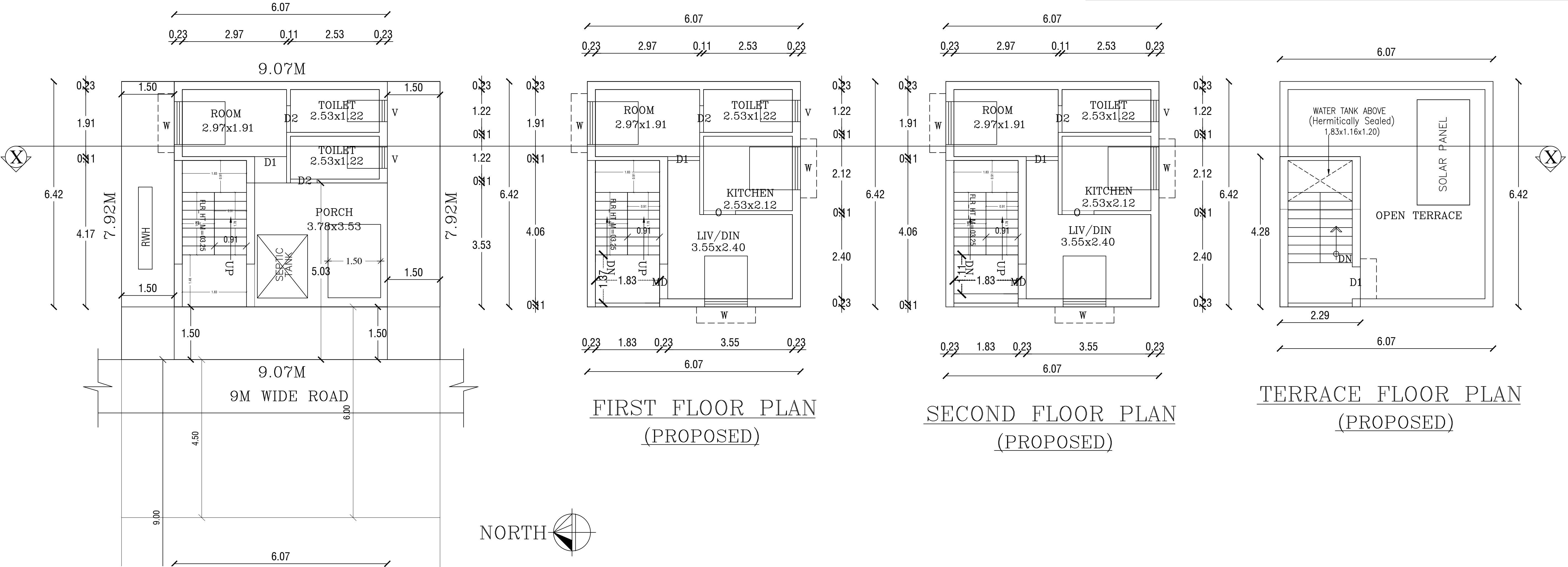
UM GROUND FLOOR PLAN (PROPOSED)
