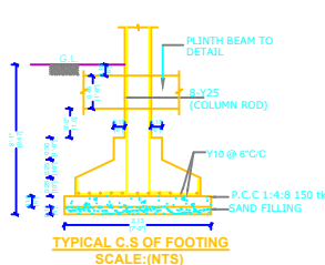
TYPICAL C.S. OF FOOTING SCALE:(NTS)
