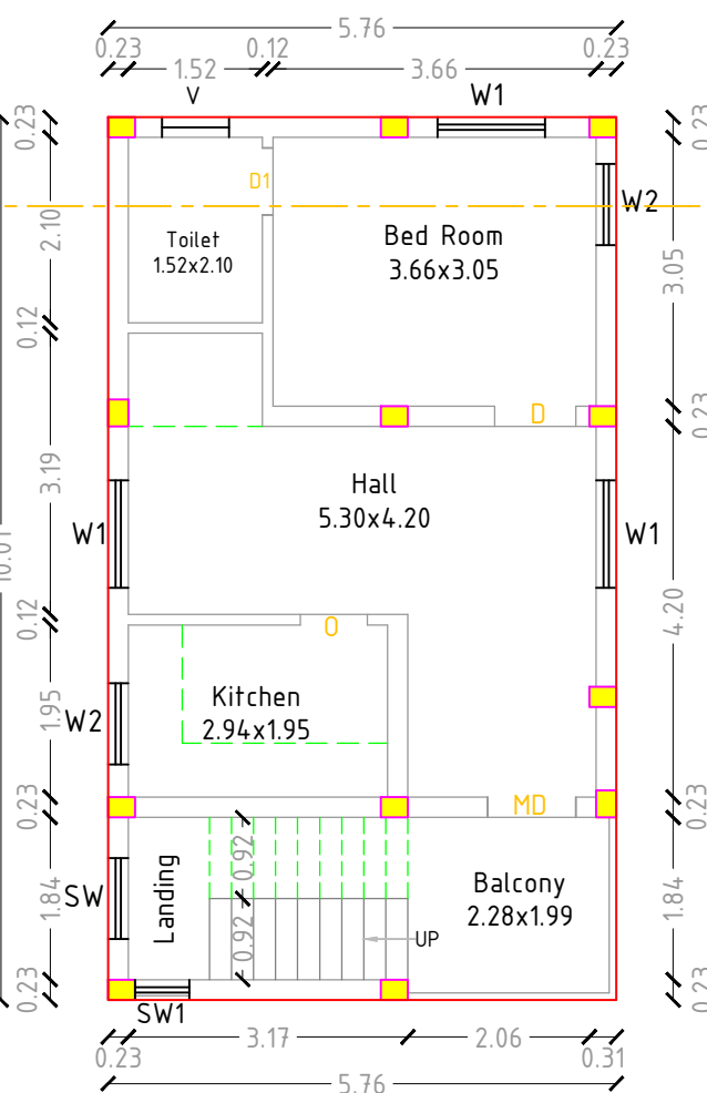
TYPICAL FLOOR PLAN FIRST & SECOND
