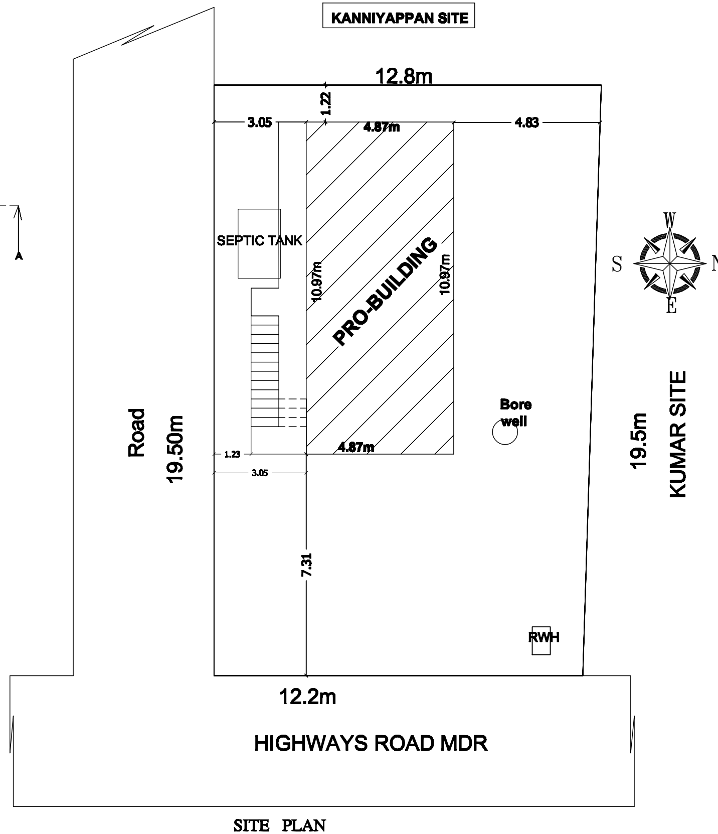
SITE PLAN
