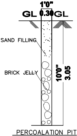
PERCOLATION PIT
