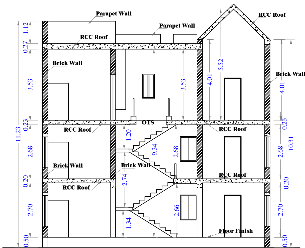
SECTION ON-AA
