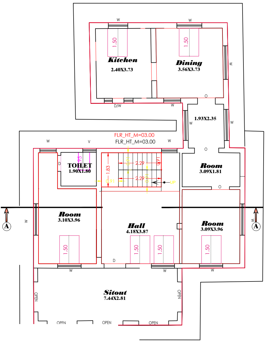
FLOOR PLAN
