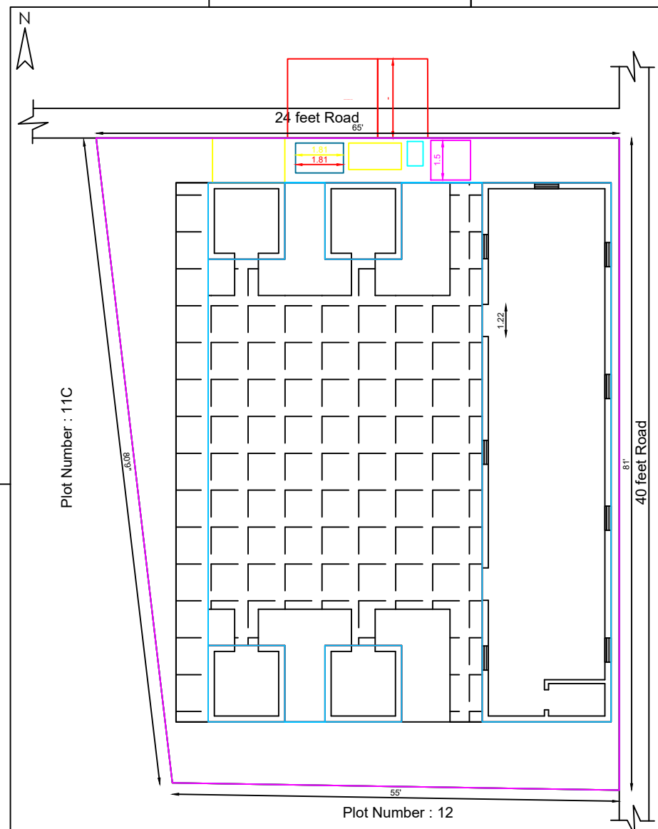
SITE PLAN
