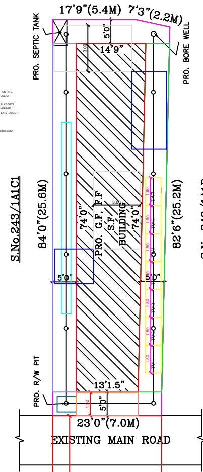
SITE PLAN
