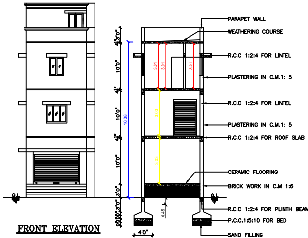
SECTION ON 'SC'
