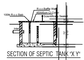
SECTION OF SEPTIC TANK "X-Y"
