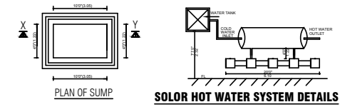
SOLAR HOT WATER SYSTEM DETAILS
