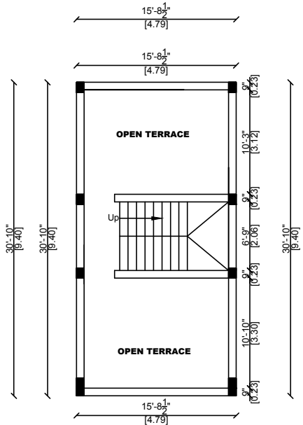
PROPOSED TERRACE FLOOR PLAN
