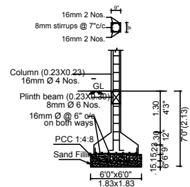
FOUNDATION DETAIL
