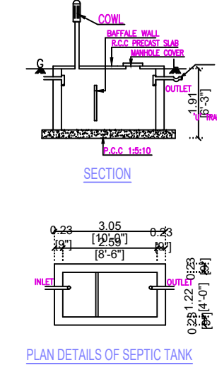
PLAN DETAILS OF SEPTIC TANK
