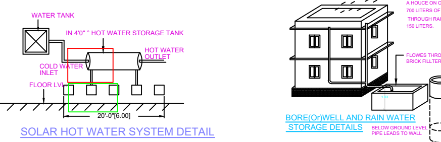
SOLAR HOT WATER SYSTEM DETAIL
