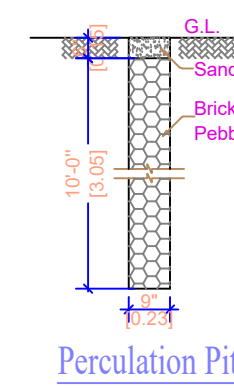
Percolation Pit
