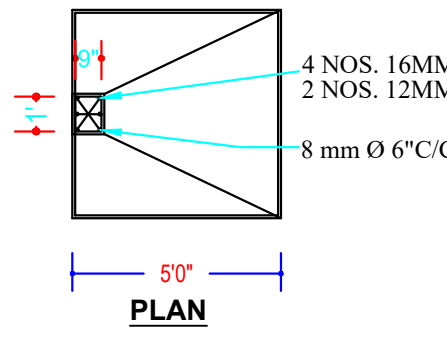
PLAN END WALL FOUNDATION
