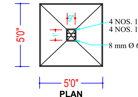
PLAN DETAIL OF COLUMN C1,C2
