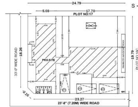
SITE PLAN [1:200]
