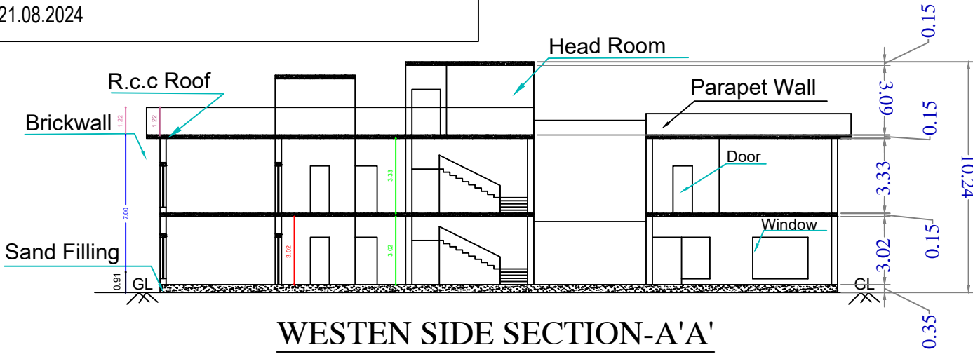
WESTEN SIDE SECTION-A'A'
