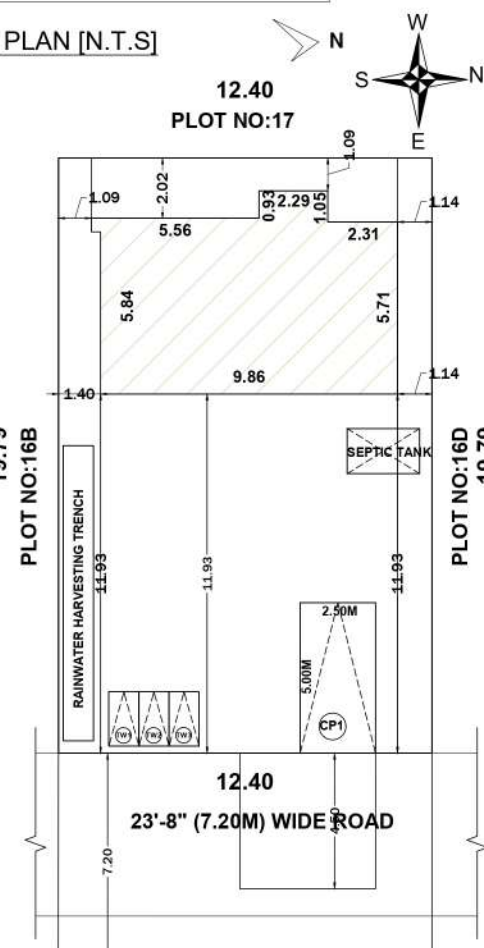
LOCATION PLAN [N.T.S.]
