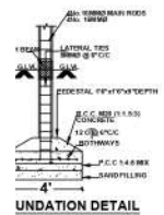
FOUNDATION DETAIL
