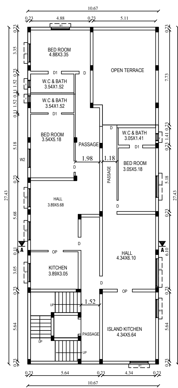
PRO.THIRD FLOOR PLAN
