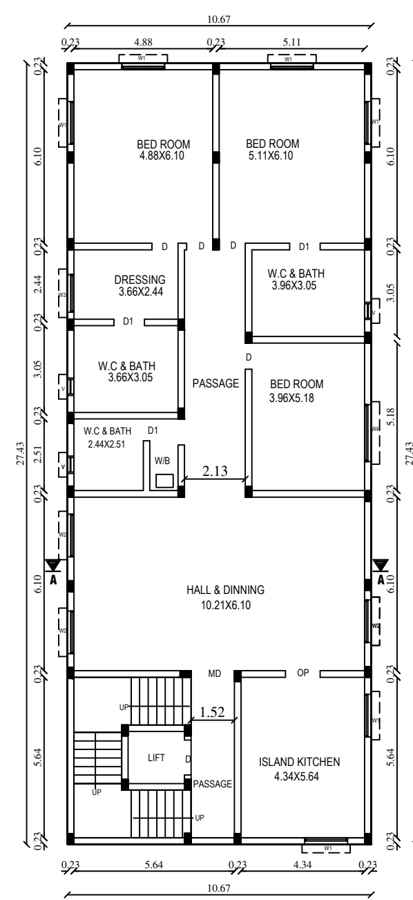
PRO.SECOND FLOOR PLAN
