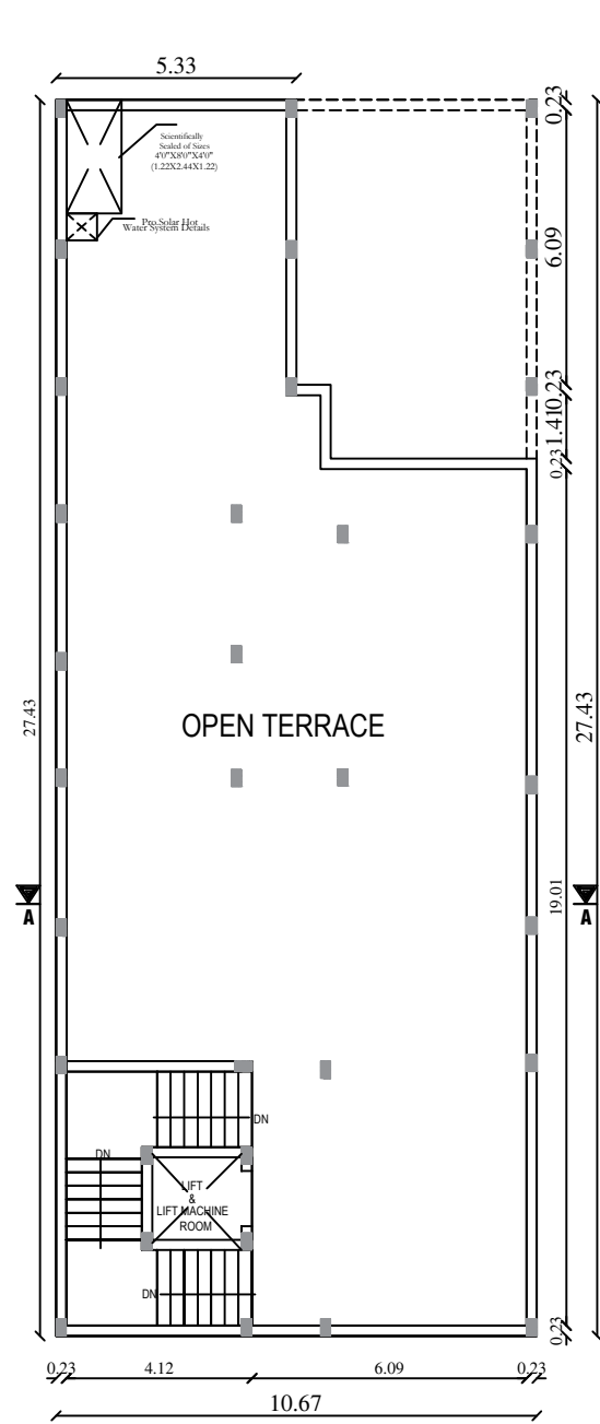
PRO.TERRACE FLOOR PLAN
