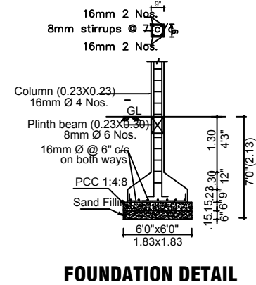
FOUNDATION DETAIL
