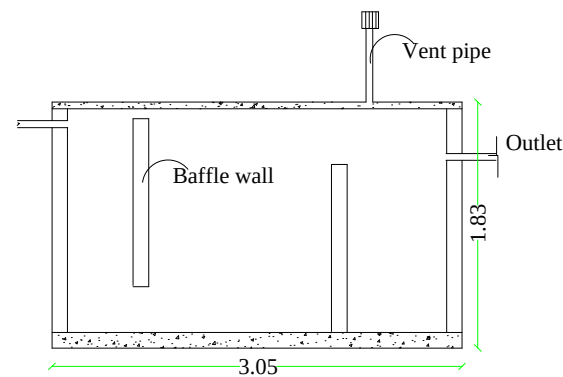
SEPTIC TANK DETAILS Size: 3.05 x 1.83 SCALE 1:100
