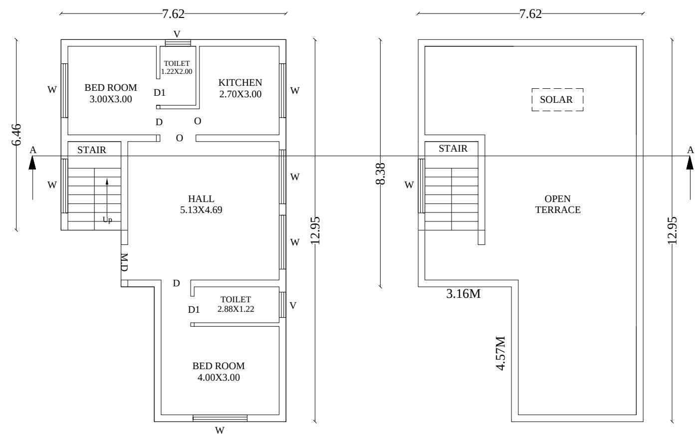
TERRACE FLOOR
