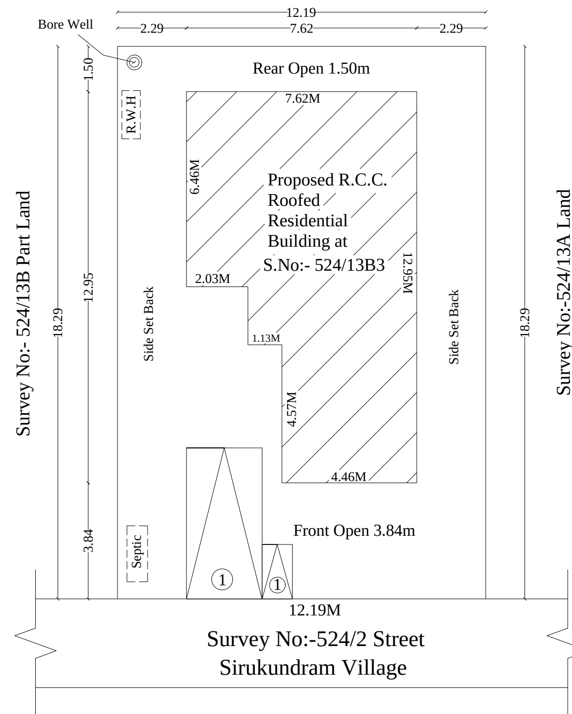
SITE PLAN
