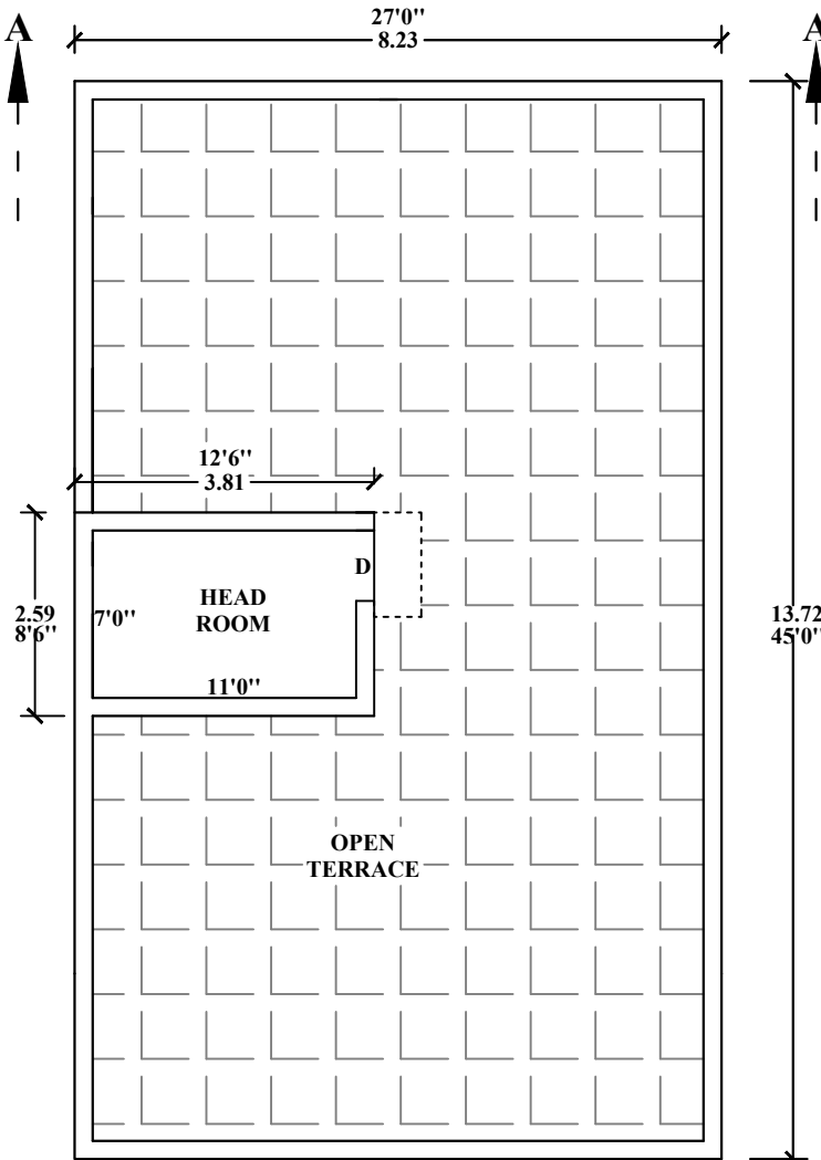
PLAN - TERRACE FLOOR
