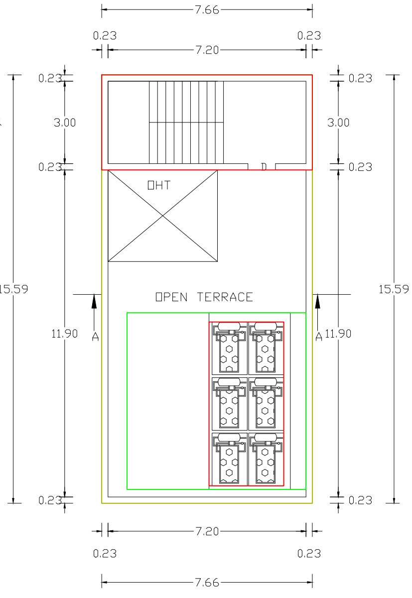
Terrace floor
