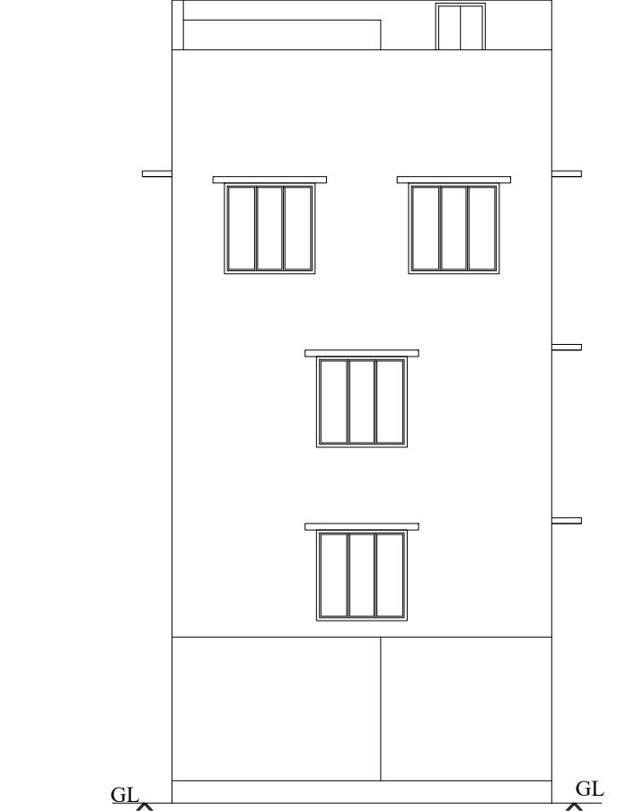
Front Elevation
