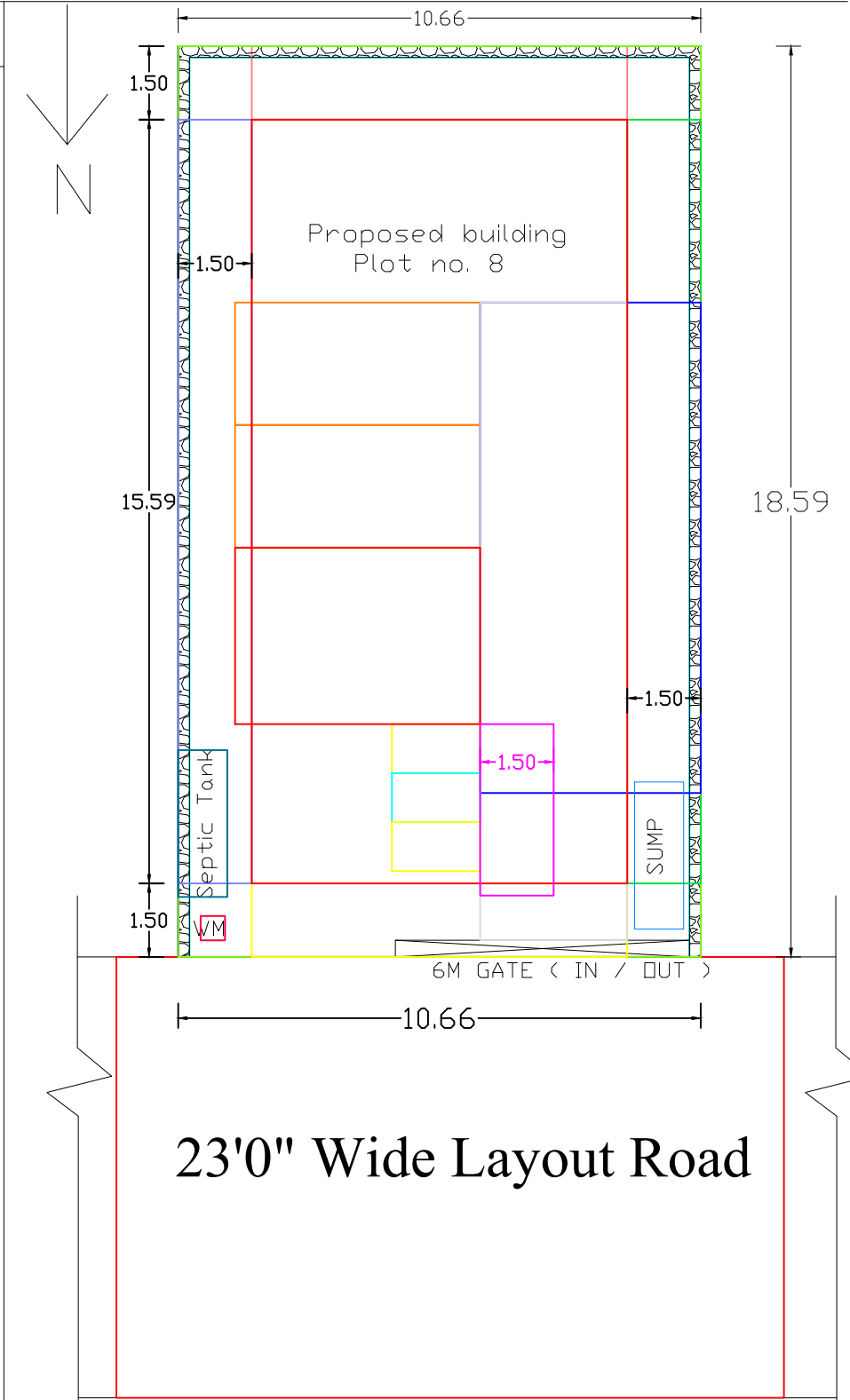
SITE PLAN
