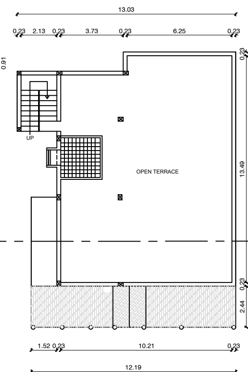
TERRACE FLOOR PLAN (EXISTING AND PROPOSED)
