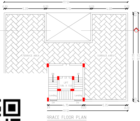
REAR FLOOR PLAN
