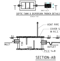
SECTION-AB
