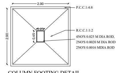
COLUMN FOOTING DETAIL
