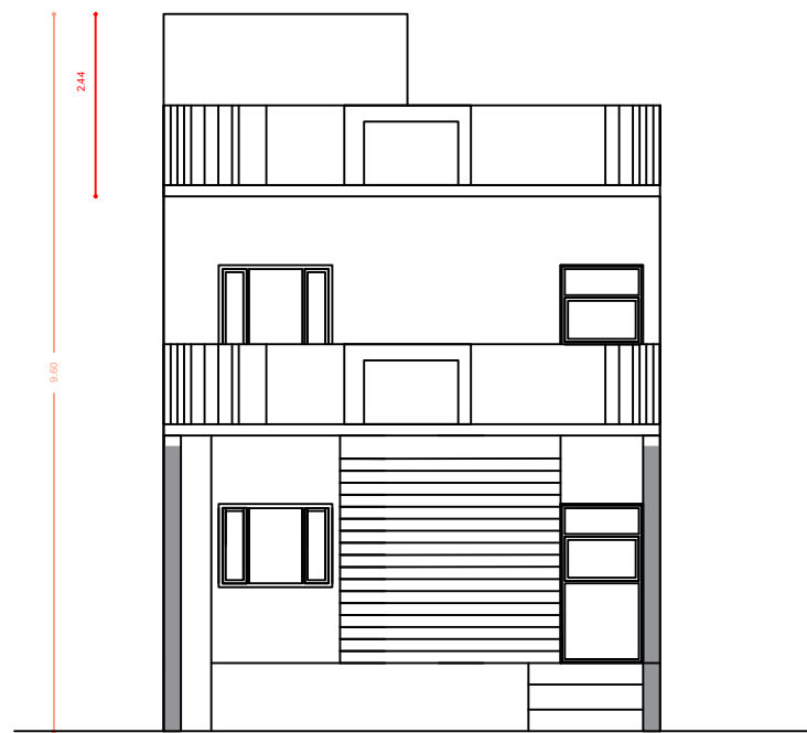
FRONT ELEVATION
