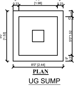
PLAN UG SUMP
