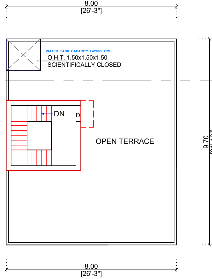
Staircase Details
