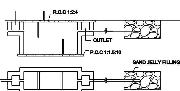
SEPTIC TANK & TRENCH
