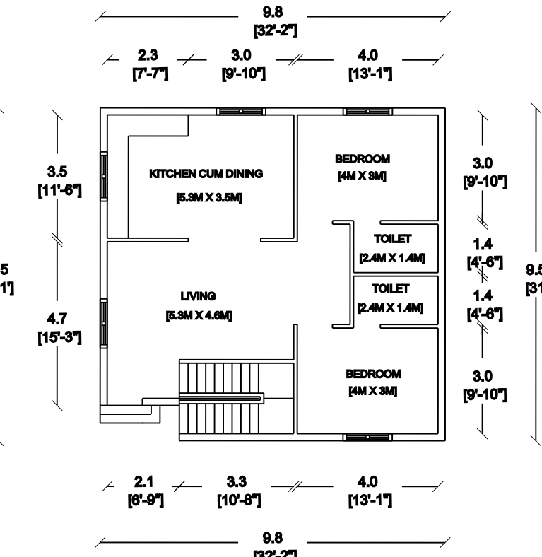
GROUND PLAN
