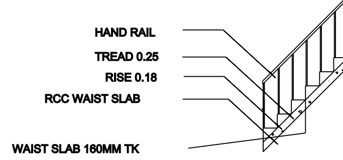
STAIRCASE DETAIL
