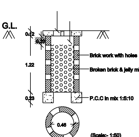
RAIN WATER
