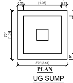
PLAN UG SUMP
