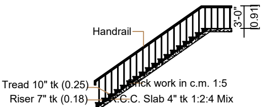
Staircase Details
