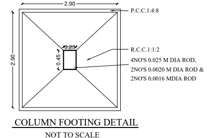
COLUMN FOOTING DETAIL NOT TO SCALE
