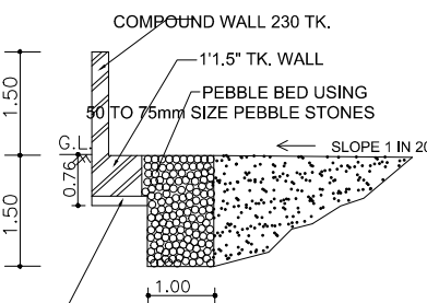
RAIN WATER COLLECTION TRENCH
