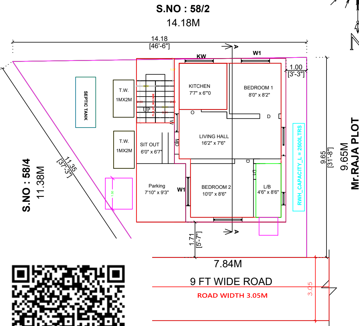
CUM GROUND FLOOR PLAN
