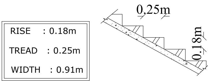
STAIRS DETAILS
