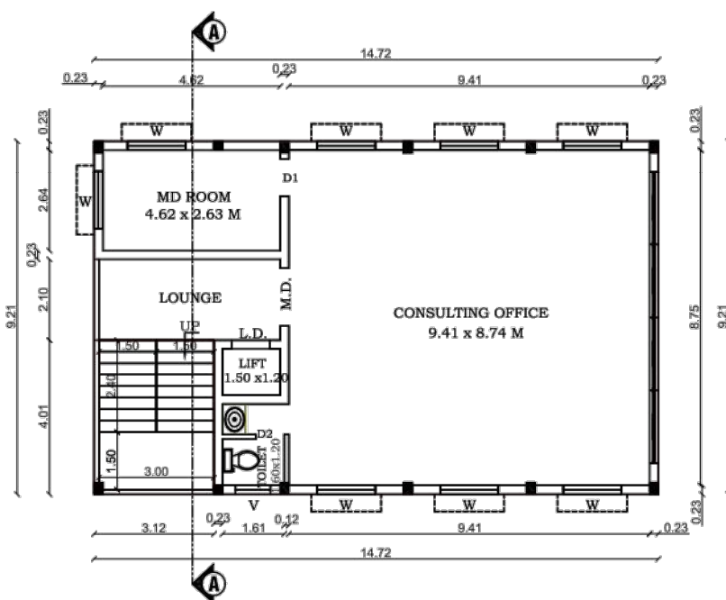
TYP. SECOND / THIRD FLOOR PLAN
