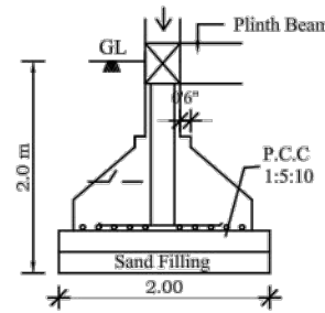
SECTION - 'CD'
