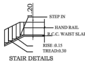
STAIR DETAILS
