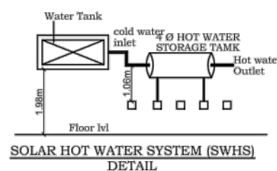
SOLAR HOT WATER SYSTEM (SWHS) DETAIL
