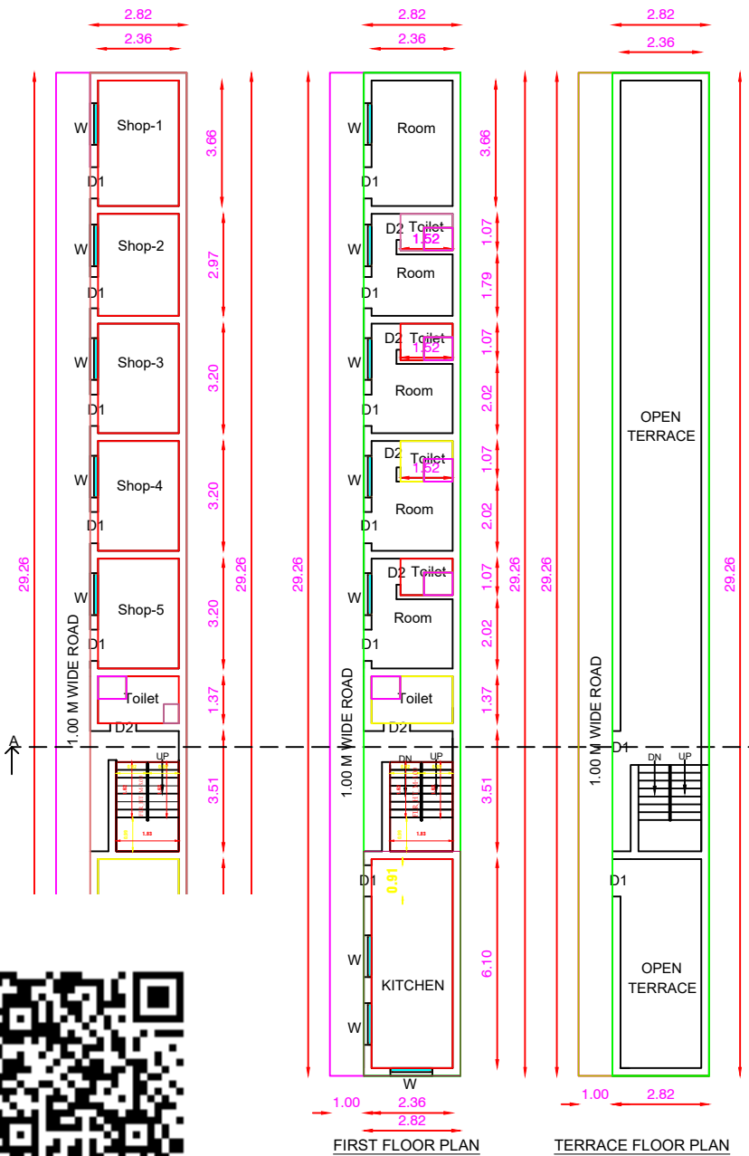
FIRST FLOOR PLAN RESIDENTIAL
