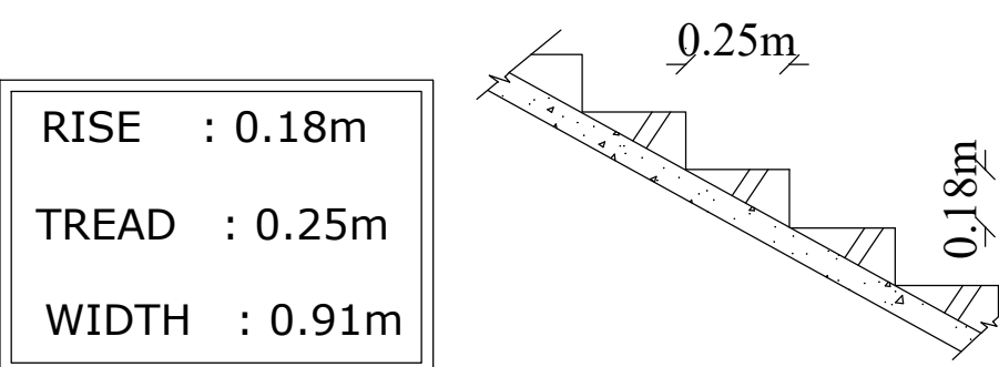
STAIRS DETAILS
