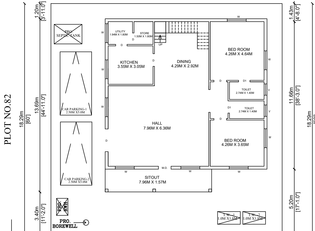
TING 40'0" WIDE LAYOUT ROAD SITE CUM GROUND FLOOR PLAN
