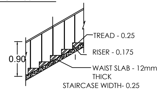
STAIR CASE DETAIL
