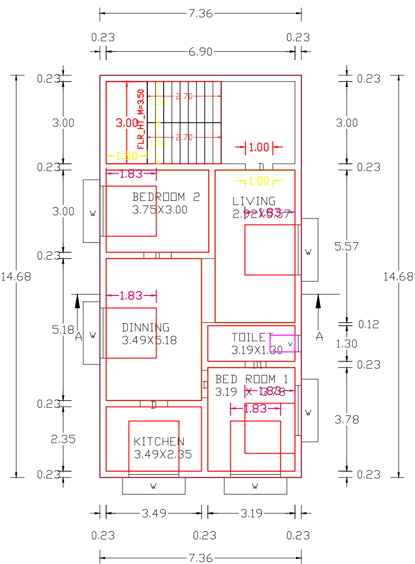
TYPICAL SECOND & THIRD FLOOR
