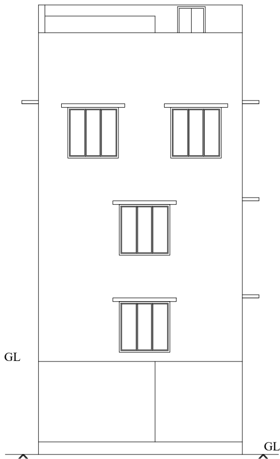
Front Elevation
