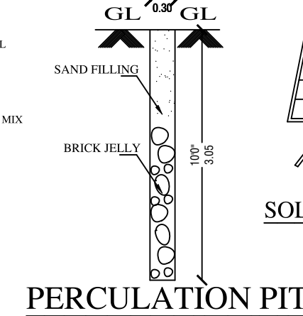
PERCOLATION PIT
