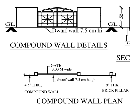
COMPOUND WALL PLAN
