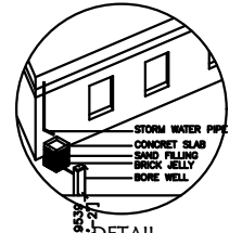
RAINWATER HARVESTING
