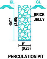
PERCOLATION PIT
