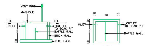
SECTION OF SEP.TANK
