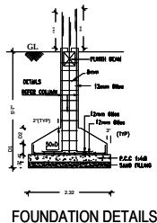
FOUNDATION DETAILS SCALE : 1:50.
