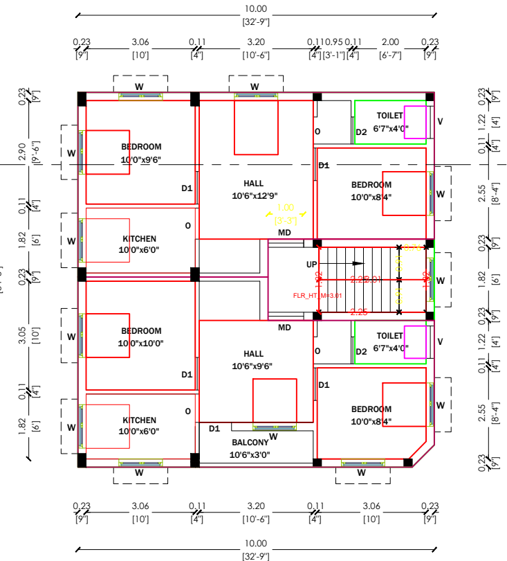
PRO. FIRST & SECOND FLOOR PLAN TYPICAL FLOOR PLAN=1,2
