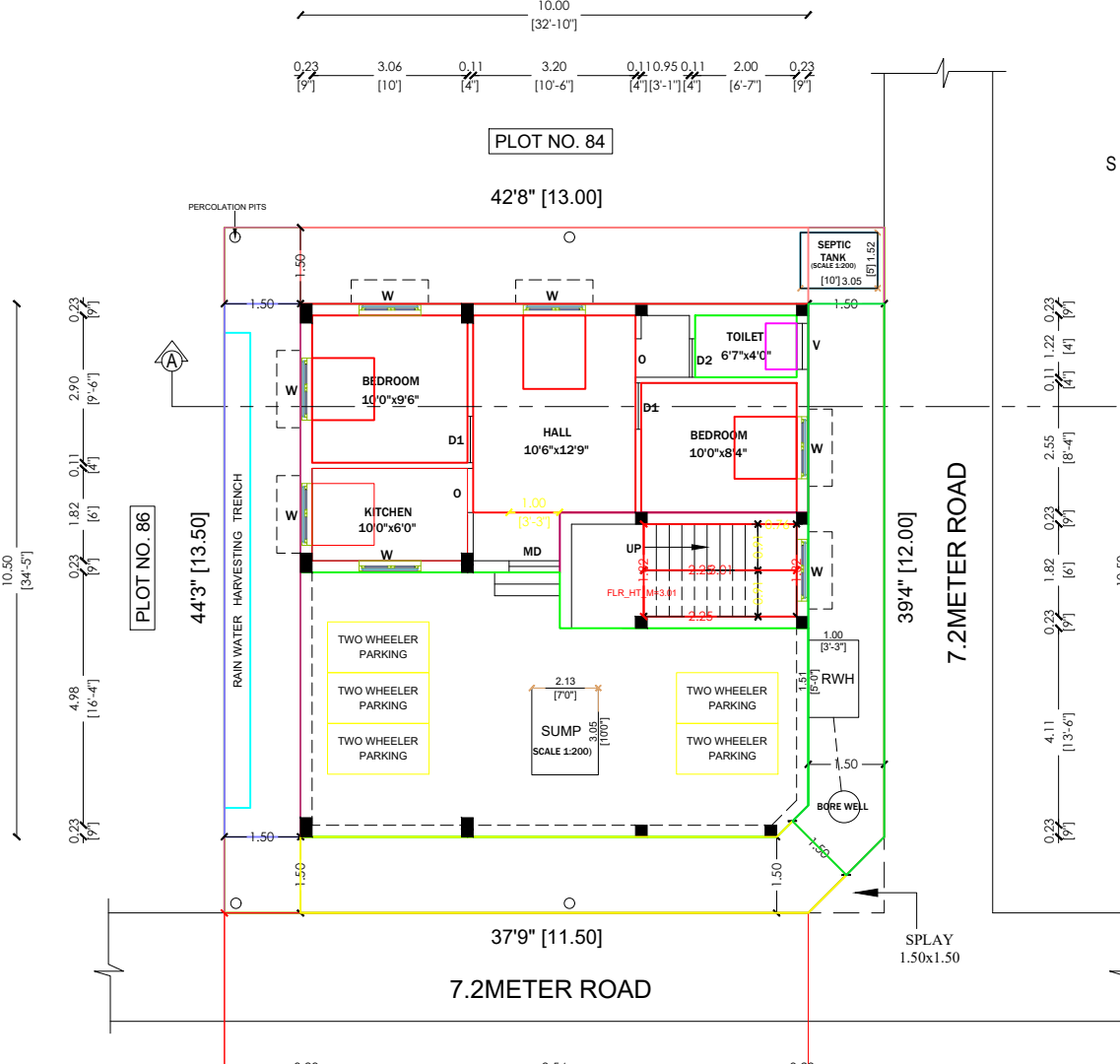
ROUND FLOOR PLAN
