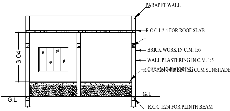
SECTION 'CC'
