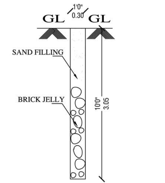
PERCOLATION PIT
