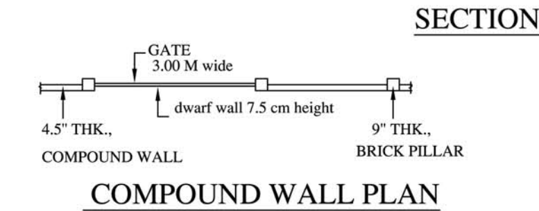
COMPOUND WALL PLAN
