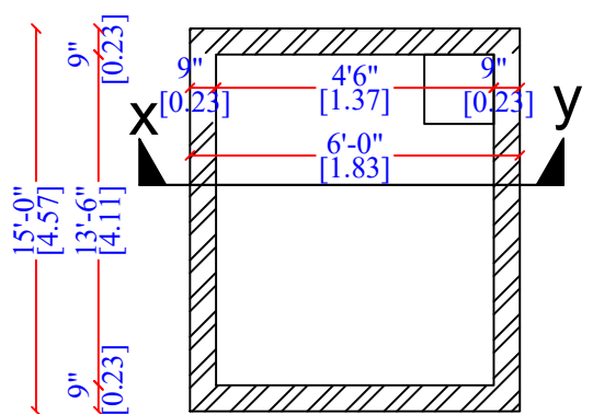
U.G.SUMP-PLAN HERMITICALLY SEALED
