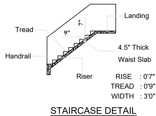
STAIRCASE DETAIL
