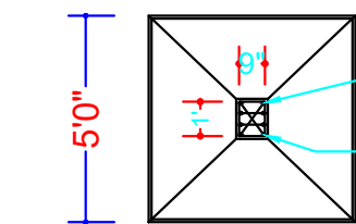
PLAN DETAIL OF COLUMN C1,C2
