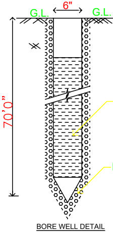
BORE WELL DETAIL
