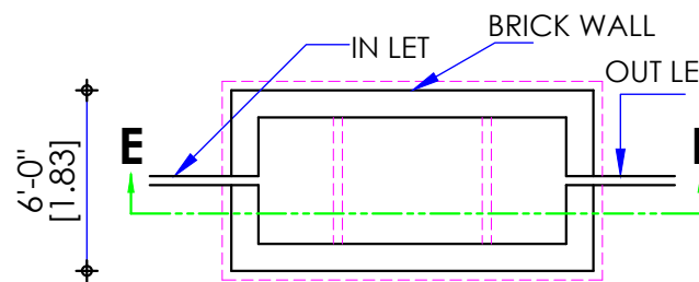
PLAN PLAN OF SEPTIC TANK
