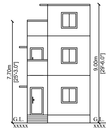
FRONT ELEVATION
