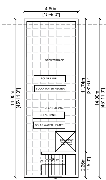
PROPOSED TERRACE FLOOR PLAN
