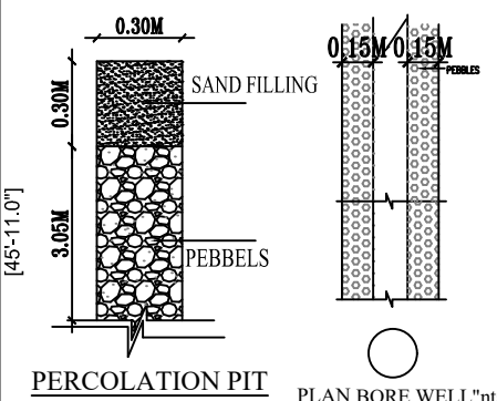
PERCOLATION PIT PLAN BORE WELL "nts
