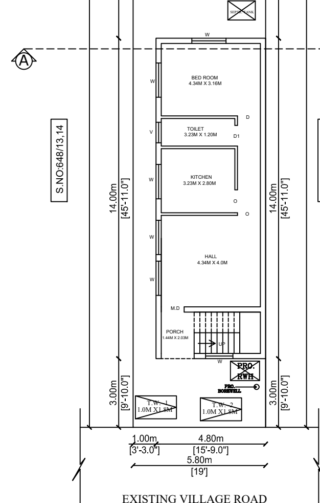
PROPOSED SITE CUM GROUND FLOOR PLAN
