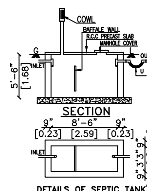
DETAILS OF SEPTIC TANK
