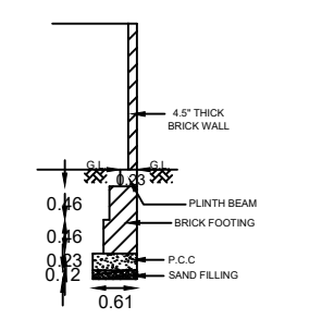
COMPOUND WALL
