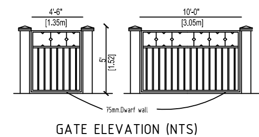
GATE ELEVATION (NTS)
