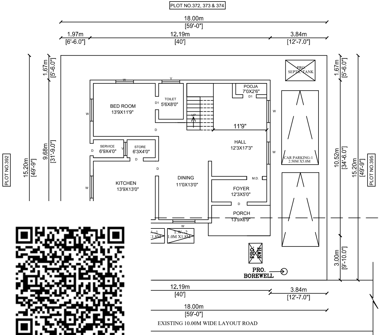
PROPOSED SITE CUM GROUND FLOOR PLAN
