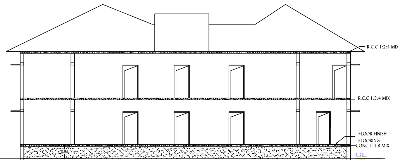
SECTION : "A-A"
