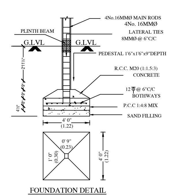
FOUNDATION DETAIL
