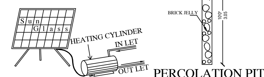
SOLAR WATER HEATING SYSTEM
