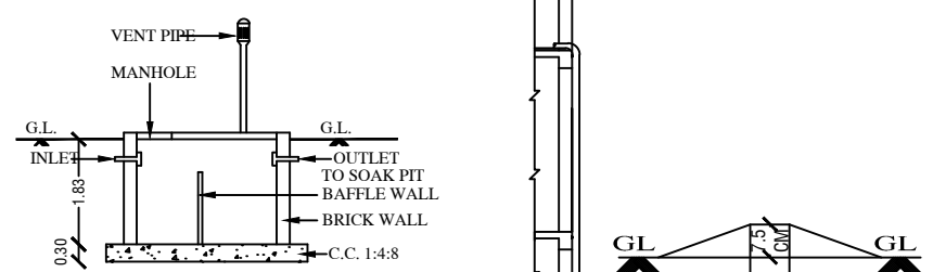
SECTION OF SEPT. TANK
