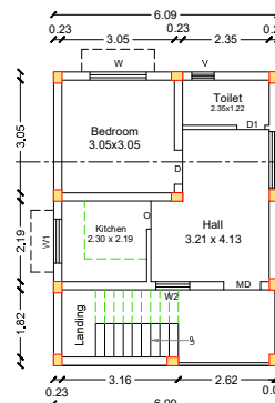
TYPICAL FLOOR PLAN SECOND AND THIRD
